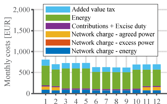
Fig. 2. Structure of electrical energy costs for an industrial consumer.
