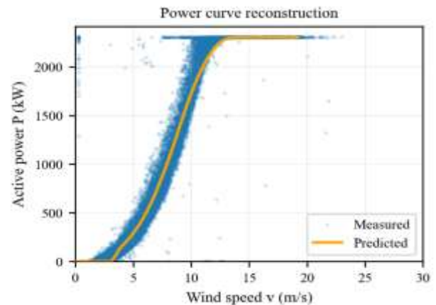
Fig.2. Reference power curve provided by the manufacturer and measured active power output.
