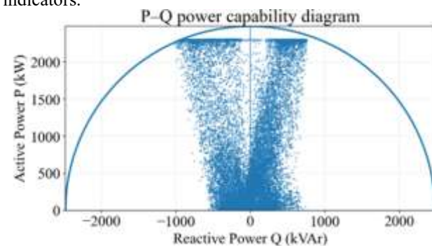
Fig.6. P-Q capability boundary for analysed WT.
