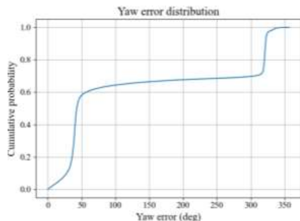
Fig.5. Cumulative distribution function (CDF) of the yaw error angle, calculated as a absolute error between nacelle position and wind direction.
