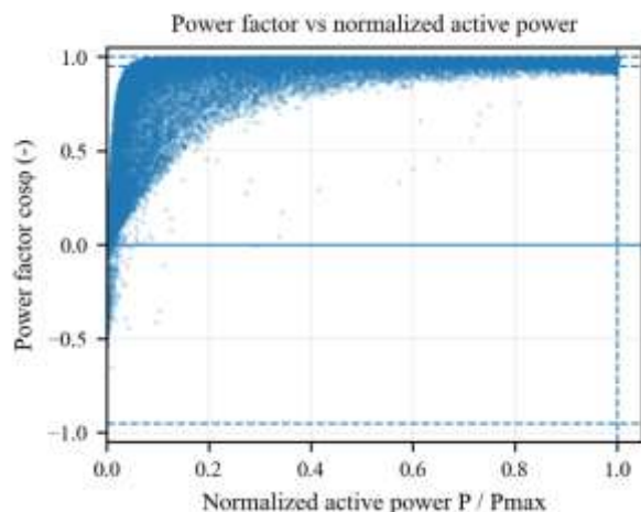
Fig.7. \cos\phi –P graph for analysed WT.
