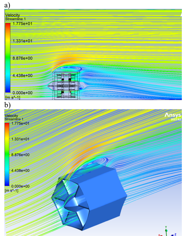
Fig.6. Flow fields in and around the device for inlet velocity 12 m/s and inertial resistance 8 m -1 .
