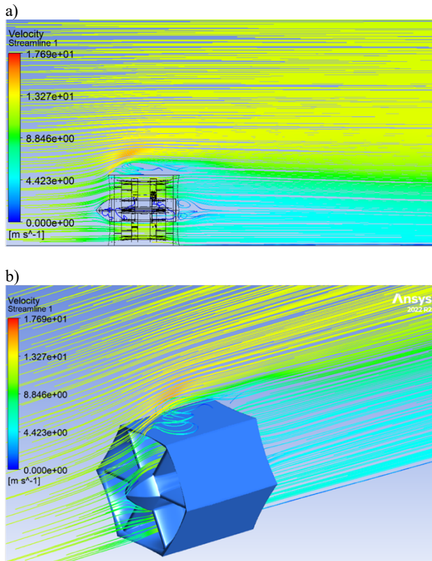
Fig.5. Flow fields in and around the device for inlet velocity 12 m/s and inertial resistance 3 m -1 .
