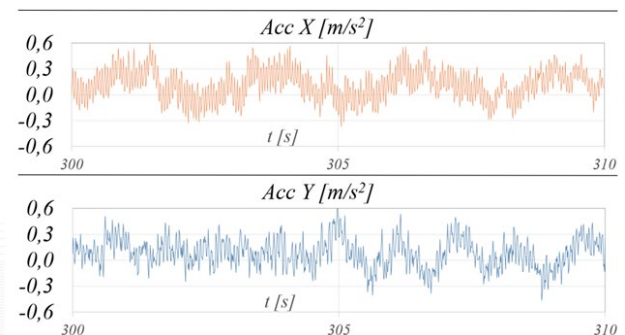
Fig. 6. Measurements of the acceleration at the nacelle: Fore-aft (up) and Side-side (down).
