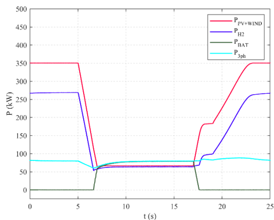
Fig. 4. Power distribution in the hybrid stand-alone plant.
