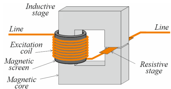
Fig. 3. Concept of operation of the IR-SFCL
