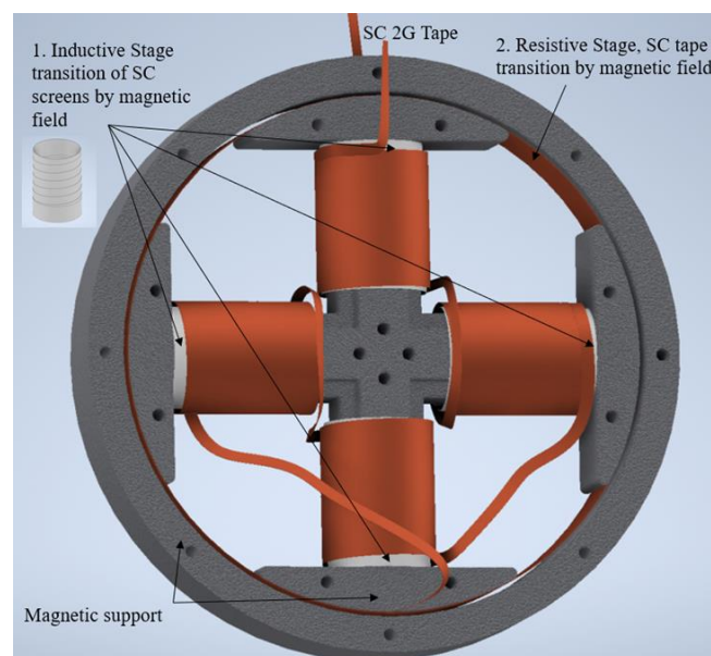
Fig. 6. Structure of the final proposed IR-SFCL
