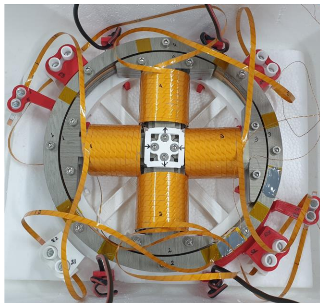
Fig. 7 Image of the IR-SFCL prototype built in the “Benito Mahedero” laboratory of Electrical Applications of Superconductors.
