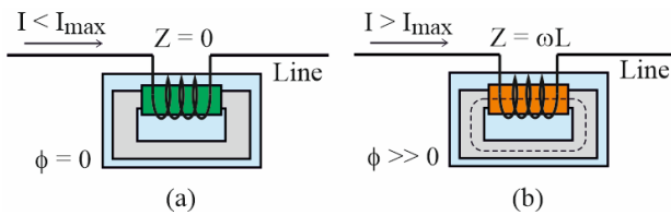
Fig. 2. Operation of the I-SFCL
