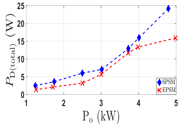
Fig. 12. Total diode losses for SPSM and EPSM under different loading conditions
