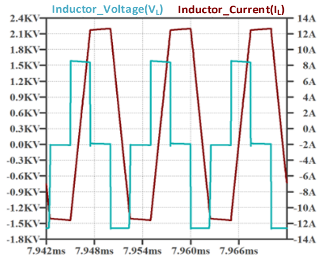
Fig. 4. Inductor Voltage and Current Waveforms of SPSM at nominal loading condition of 5 kW
