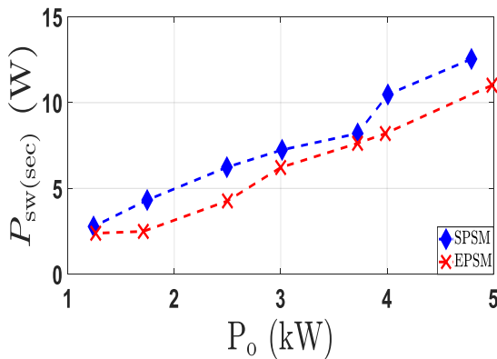
Fig. 8. Secondary-side S_5 MOSFET losses for SPSM and EPSM under different loading conditions
