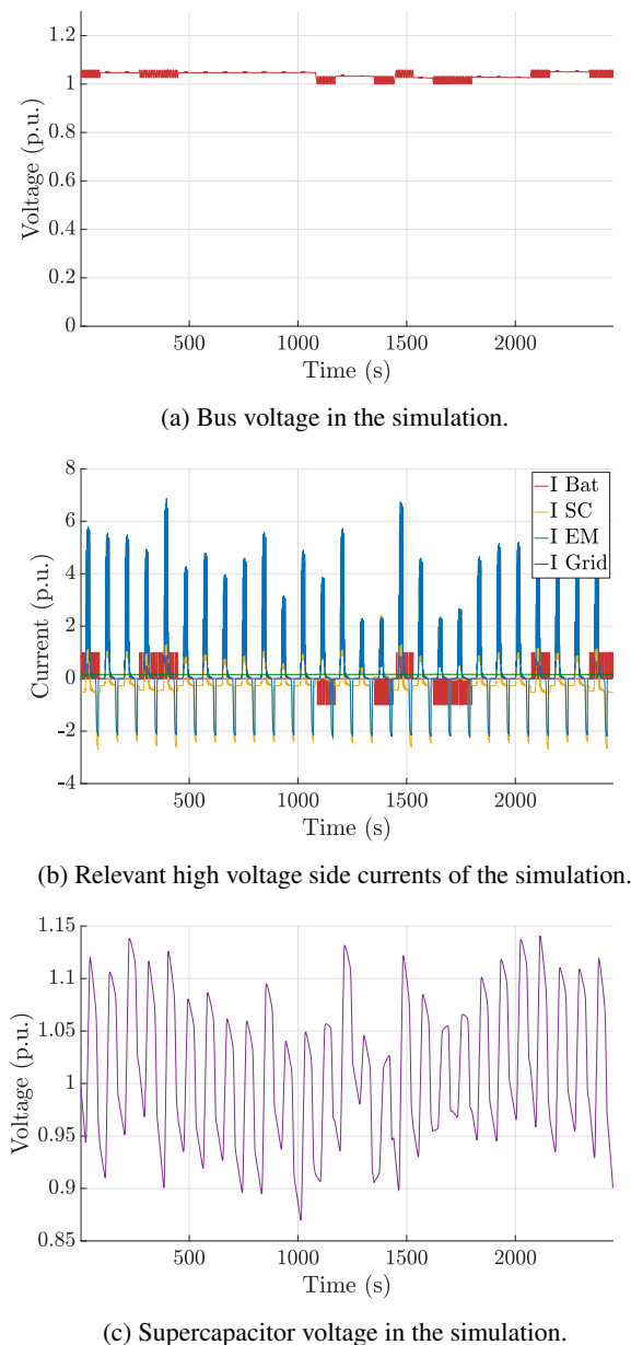
Figure 8: Simulation results over many AWES cycles.
