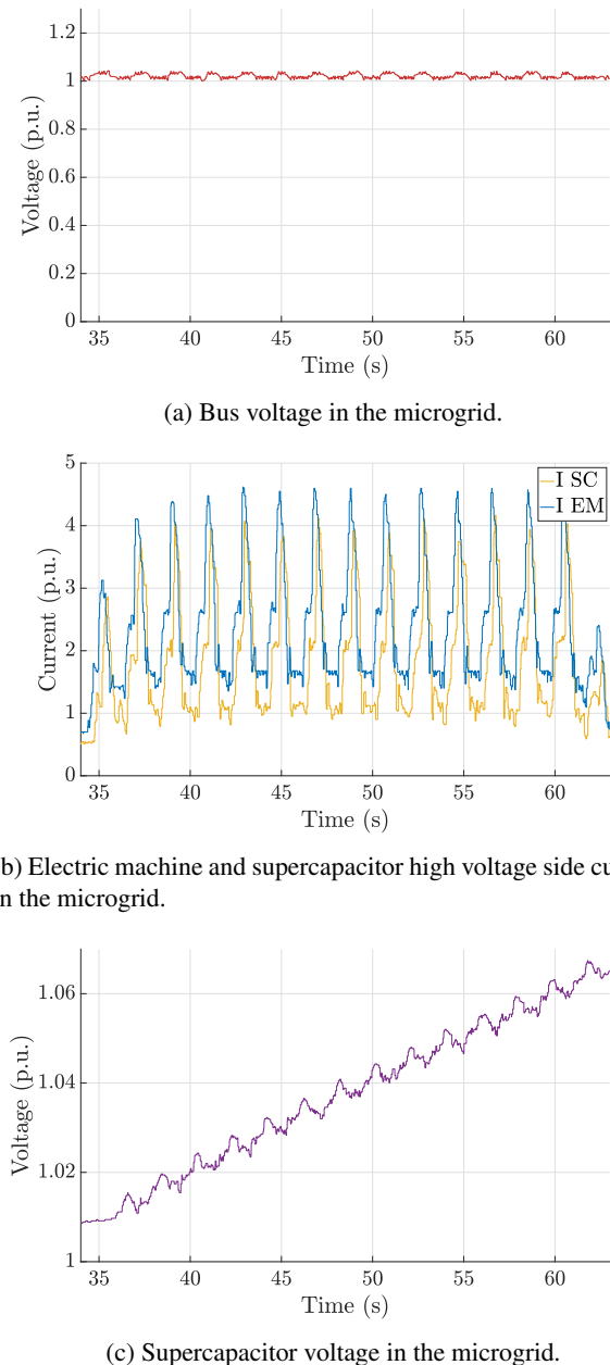
Figure 9: Results over an AWES reel-out.
