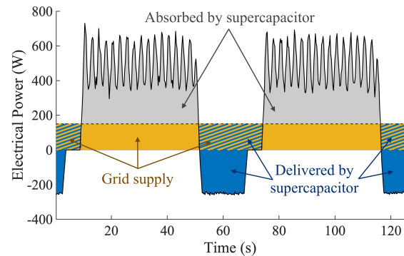
Figure 5: Conceptual representation of power flows among microgrid components during a reel-out and reel-in cycle.
