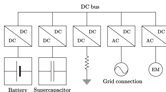
Figure 4: Proposed electric topology for AWES power conversion.
