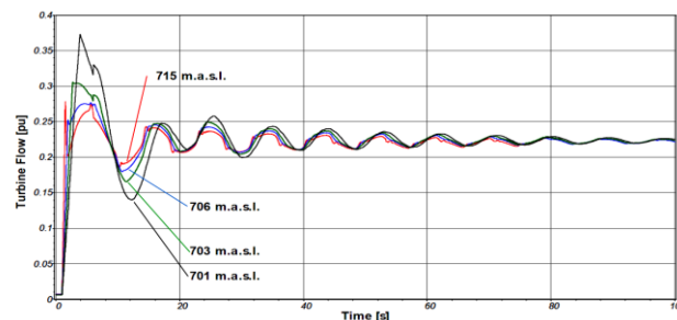
Fig. 10. Turbine water flow after a wind generator trip for different upper reservoir levels (100 s) after a 2.3 MW wind generator trip [13].
