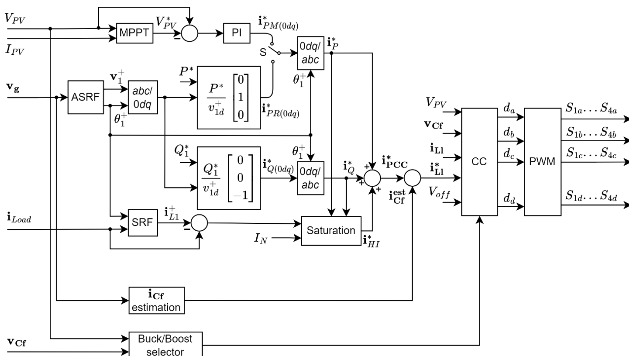
Figure 2. Block diagram of the inverter control system.
