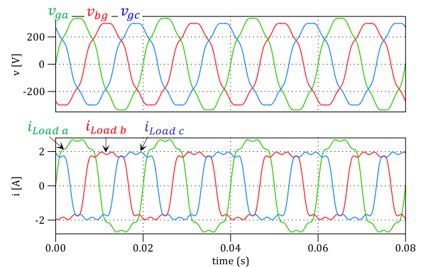
Figure 3. Top: Phase-to-neutral grid voltages distorted and unbalanced according to the limits indicated in [14] and [15]. Bottom: Unbalanced and non-linear load currents.
