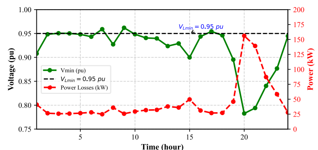
Fig. 6. ITQ feeder power losses and minimum voltage profiles without PVS.
