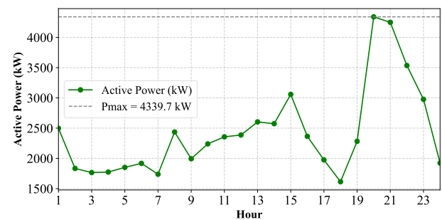
Fig. 5. Power Demand Profile.
