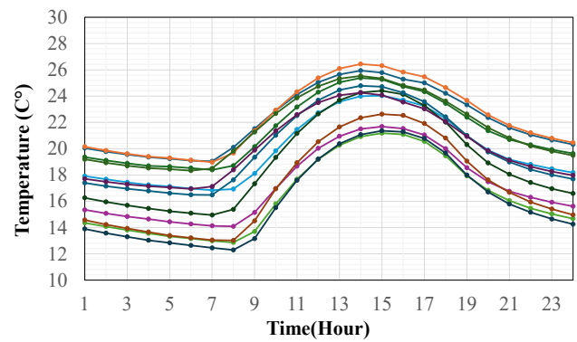
Fig. 4. Temperature Profile per month
