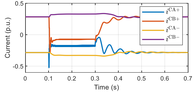
Fig. 5. Converter currents in a fault type A+ with R = 0.1 \Omega
