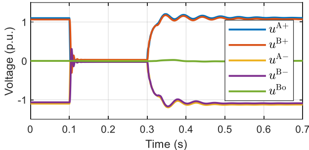
Fig. 8. Node voltages in a fault type AA with R = 0.1 \Omega
