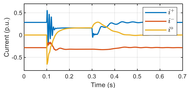
Fig. 7. Line currents in a fault type Bo+ with R = 0.1 \Omega
