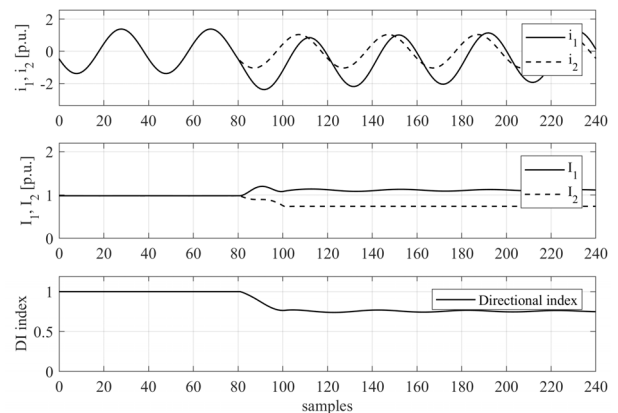
Fig. 7. 10% Interturn fault case for PT positioned between the active and passive networks
