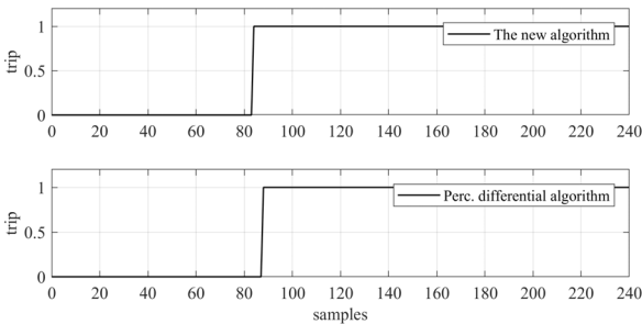
Fig. 10. 50% Interturn fault case: trip decisions for PT positioned between the active and passive networks
