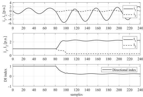
Fig. 9. 50% Interturn fault case for PT positioned between the active and passive networks
