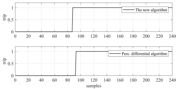
Fig. 8. 10% Interturn fault case: trip decisions for PT positioned between the active and passive networks
