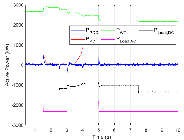
Fig. 2. Power exchange with the local grid ( P_{PCC} ) and the generated and consumed power in the MGC.
