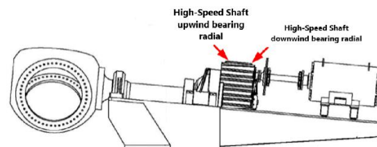
Fig.1. Location of vibration measurement sensors [3].
