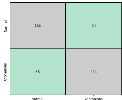
Fig.5. Confusion matrix for data error detection of the High-Speed Shaft downwind bearing radial sensor.
