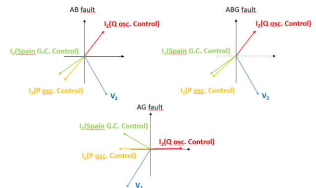
Fig.11. Comparison of I2 current injection for the three different controls.
