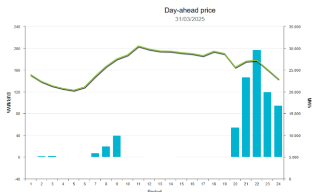
Fig. 12. Average electricity prices, March 31 st , 2025 [7]
