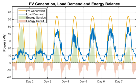
Fig. 6. Photovoltaic generation and consumption profiles for Scenario I.
