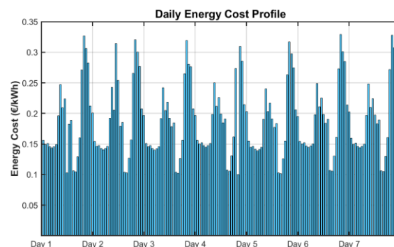
Fig. 5. Energy cost profile.
