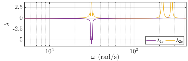
Fig. 4. Eigenvalues obtained to check the passivity of the GFL converter.
