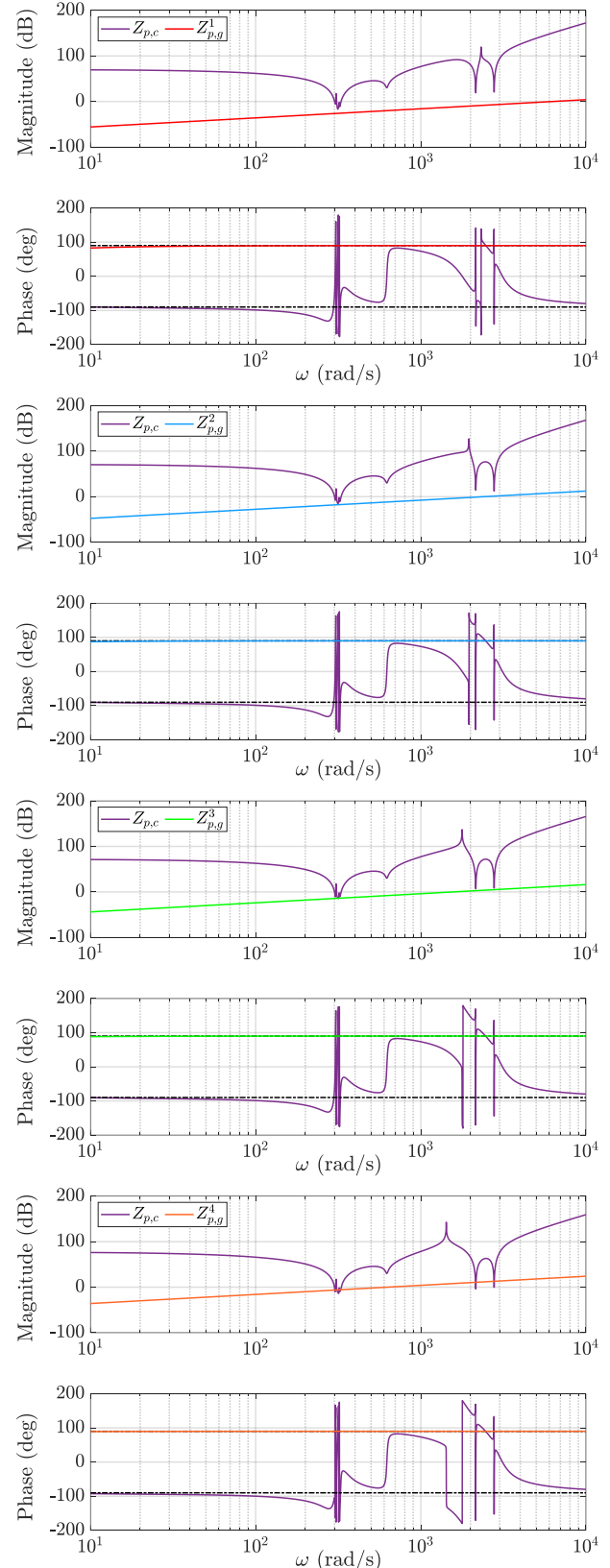
Fig. 7. Positive-sequence impedances of the GFL-grid systems.
