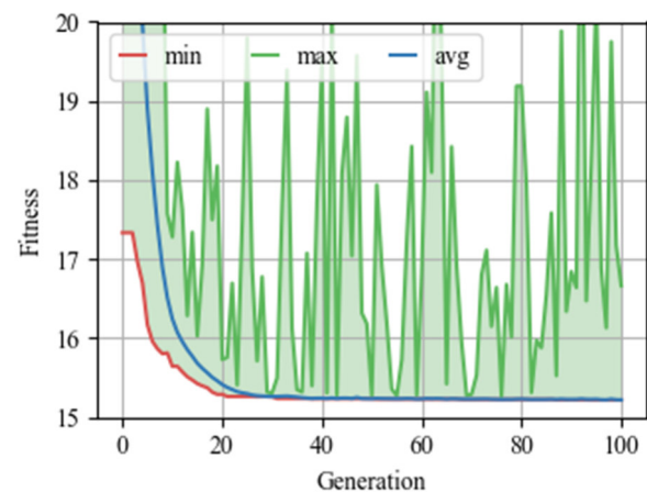
Fig.3. Evolution of the proposed genetic algorithm with hyperparameters p_{cx} = p_{mut} = 0.5 .
