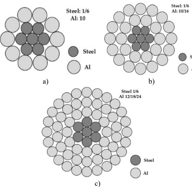
Figure 1. Cross Section Schematics of a). single layer b). two layer and, c). three layer conductor
