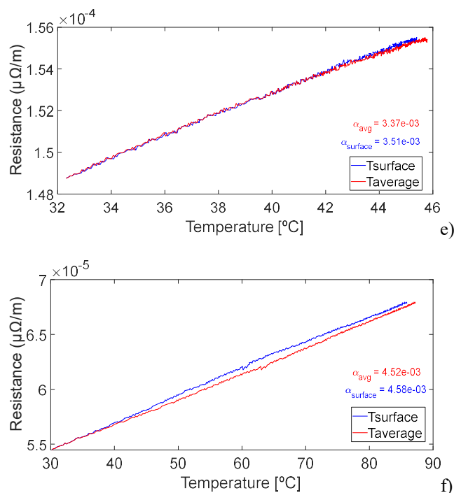
Figure 3. Temperature change and temperature coefficient of resistance for single-, two-, and three-layer conductors. Subfigures 3a, 3b, and 3c show the surface, core, and average temperatures, while subfigures 3d, 3e, and 3f show the \alpha_{surface} (experimental) and \alpha_{avg} (simulated) values for single-, two-, and three-layers conductors respectively.
