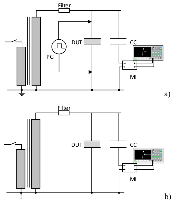
Figure 2. a) Circuit calibration. b) Background noise level measurement.
