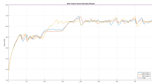
Fig.7. Power output of each wind turbine after 6 iterations of training.
