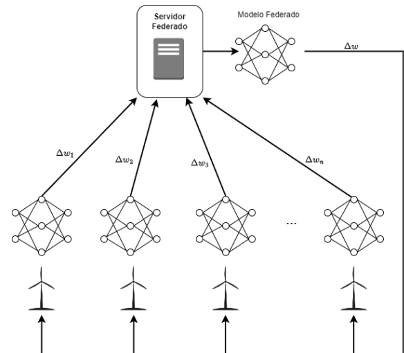
Fig.2. Federated learning scheme applied to wind turbines.
