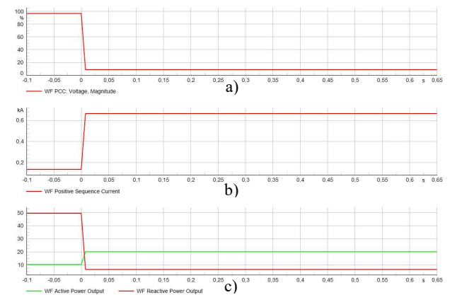
Fig. 5. Three phase Fault 1. a) PCC positive sequence voltage (%), b) WF positive sequence current (kA), c) WF Active power (MW) and Reactive power (MVar) output.
