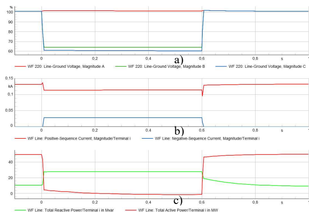
Fig. 13: Two phase Fault 3. Only I_2 injection. a) PCC phase voltages (%), b) WF positive & negative sequence current (kA), c) WF Active power (MW) and Reactive power (MVar) output.
