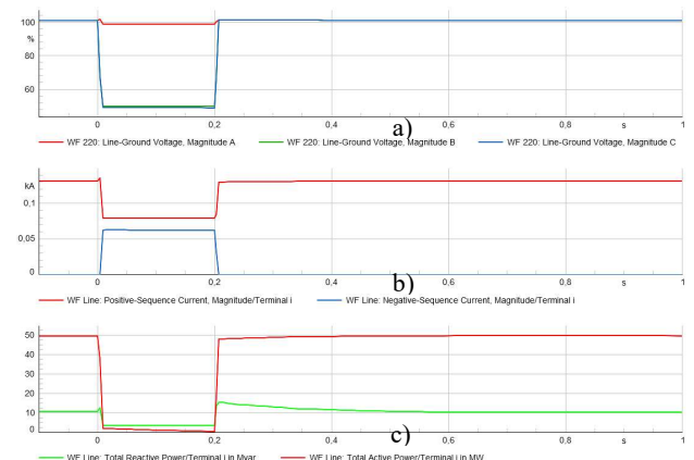
Fig. 9. Two phase Fault 1. I_1 & I_2 injection. a) PCC phase voltages (%), b) WF positive & negative sequence current (kA), c) WF Active power (MW) and Reactive power (MVar) output.
