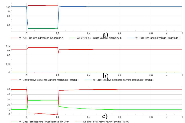
Fig. 8. Two phase Fault 1. Only I_1 injection. a) PCC phase voltages (%), b) WF positive & negative sequence current (kA), c) WF Active power (MW) and Reactive power (MVar) output.
