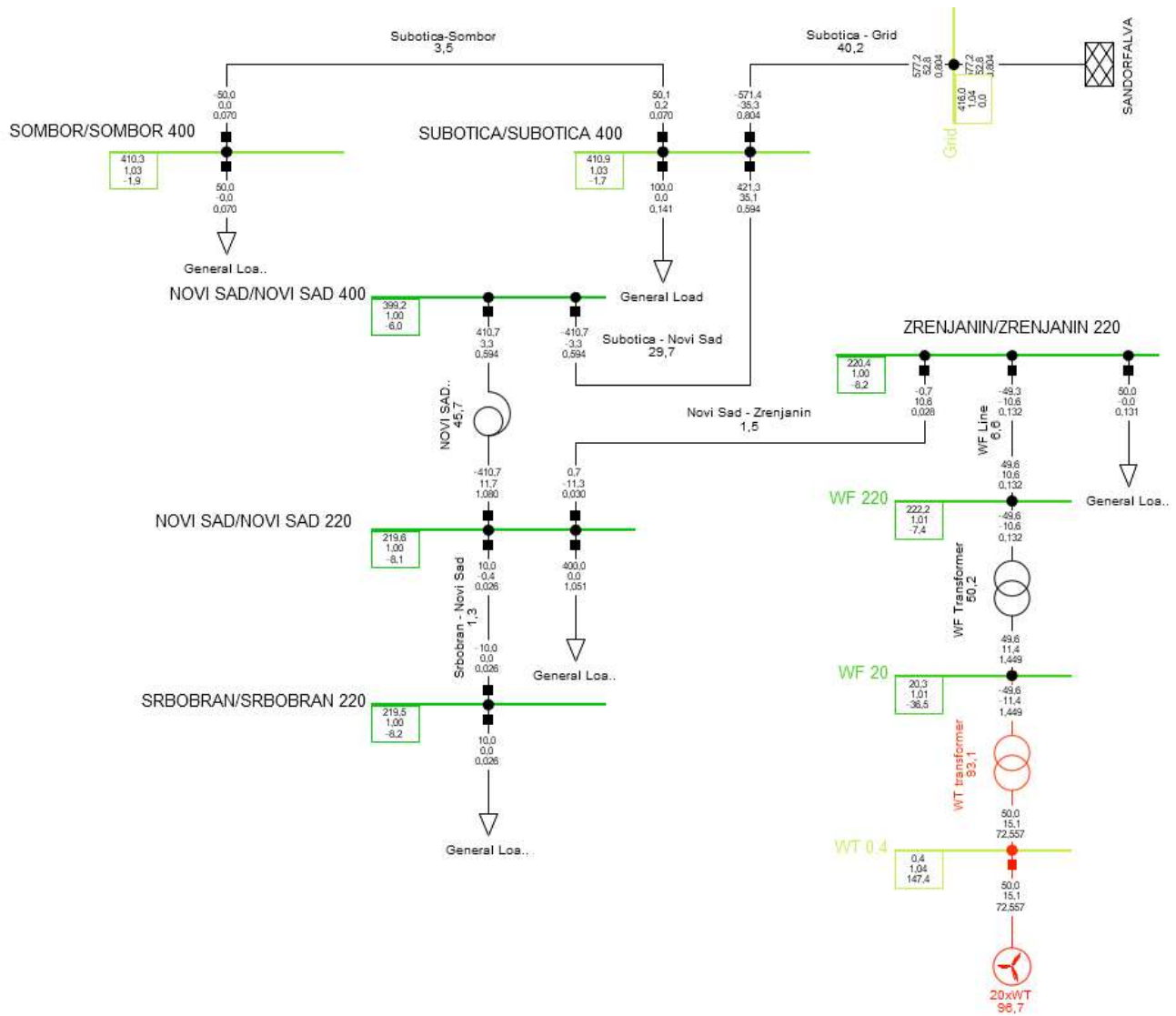
Fig. 4. DiGSILENT model after full active power load flow solution.
