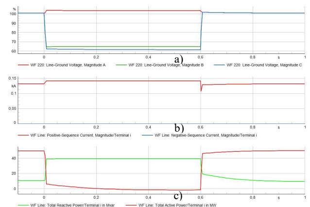
Fig. 10. Two phase Fault 3. Only I_1 injection. a) PCC phase voltages (%), b) WF positive & negative sequence current (kA), c) WF Active power (MW) and Reactive power (MVar) output.
