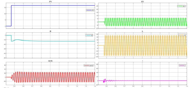
Fig.4. Current of each element of the nZEH in Scenario 2.
