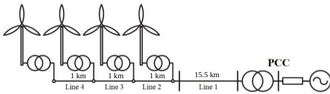
Fig. 2. Scheme of the wind farm under study.
