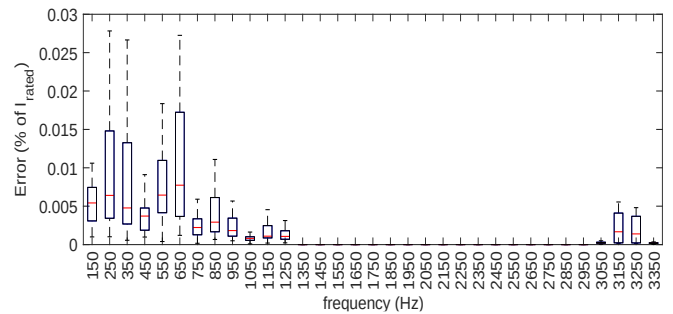
Fig. 6. Boxplot of the magnitude error of the harmonic current emission obtained by SM versus the frequency.
