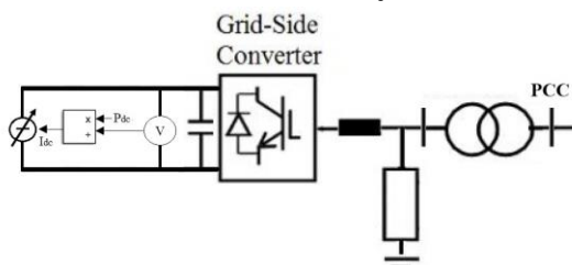
Fig. 4. Simplified scheme of the wind turbine under study.
