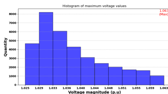
Fig. 4. 1-year long time series results - maximum voltage
