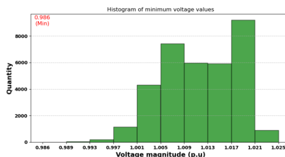
Fig. 3. 1-year long time series results – minimum voltage
