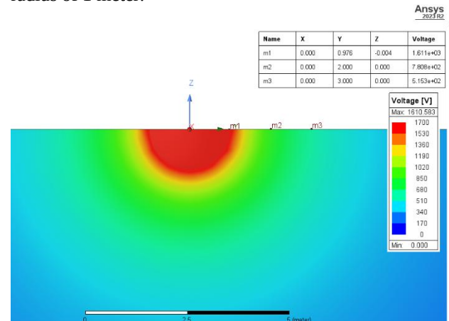
Fig. 4. Fem simulation of a hemispherical electrode
