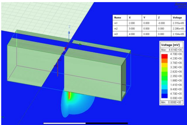
Fig. 7. Electric Potential Distribution near the Tunnel with One Vertical Rod and a Private Earth Electrode Spaced 3 m apart
