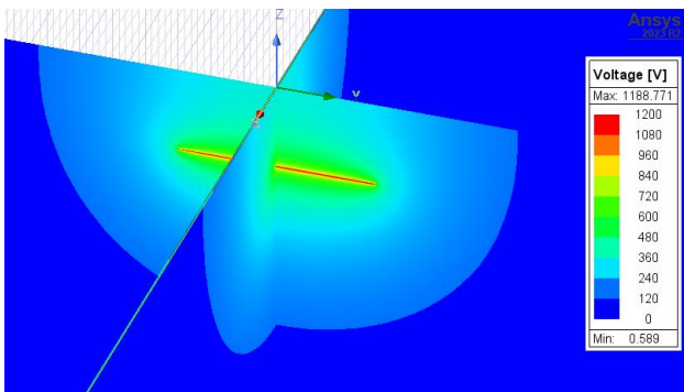
Fig. 6. Potential distributions for buried copper conductor
