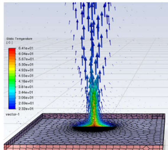
Fig. 3. Heat loss due to free convection.
