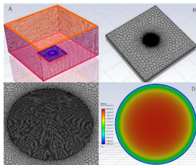
Fig. 2. CFD simulation of the experimental: Meshing (A, B, C) and temperature distribution on sample top surface (D).
