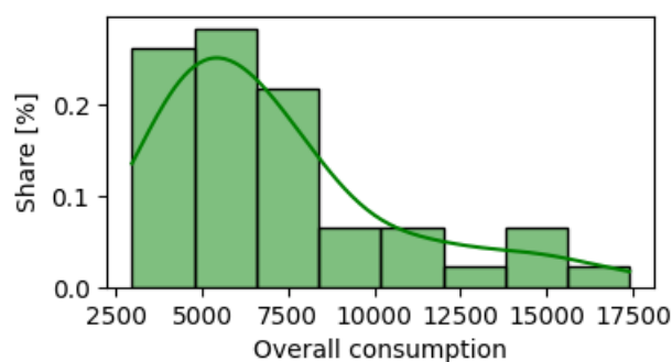
Fig.4. Histogram of prosumers overall consumption
