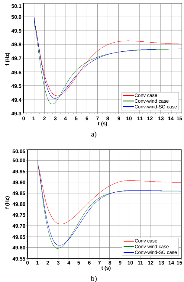
Fig. 4. System frequency time evolution for a sudden disconnection of the Diesel 9 generator unit of Punta Grande power plant for conv case, conv-wind case and conv-wind-SC case ( H_{SC} = 2 MWs/MVA): a) off-peak demand state; b) peak demand state.
