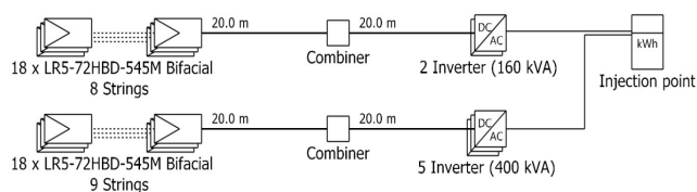
Figure 3. Bifacial PV String and Inverter Configuration for Grid Injection
