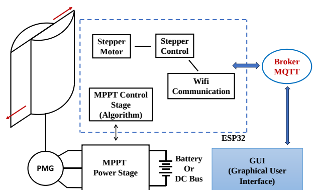
Figure 12 : Block diagram of the developed system
