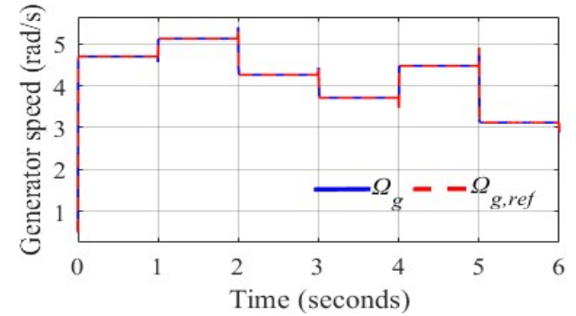
Fig. 14. Generator speed \Omega_g .
