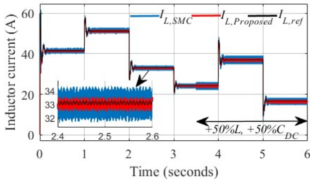
Fig. 16. Inductor current.
