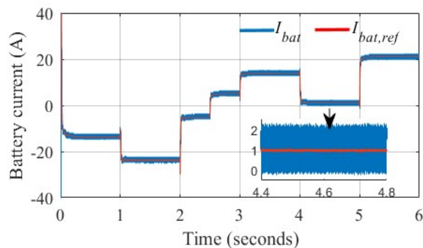
Fig. 21. Battery current.
