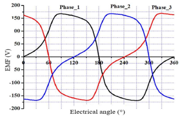
Fig. 7. DSPM electromotive force.
