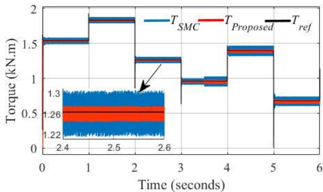
Fig. 18. Generator electromagnetic torque.
