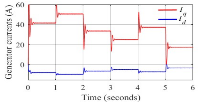
Fig. 15. Generator current.
