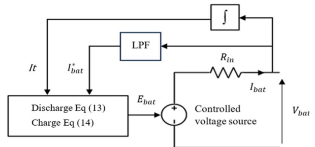
Fig. 11. Equivalent circuit of the lithium-ion battery model.
