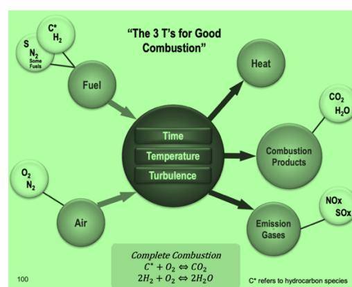
Fig. 11 Complete combustion cycle
