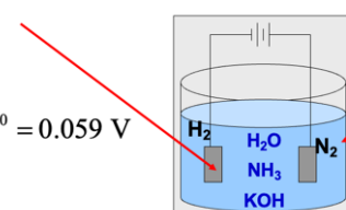
Fig. 9 Ammonia Oxidation reaction
