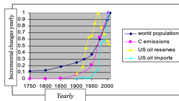
Fig.1 World population, World carbon dioxide emissions-(Source IEA)
