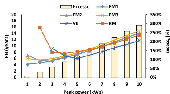
Fig. 4. Payback (DET 4)
