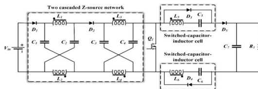
Fig. 1. Two cascaded Z-source high step-up converter.
