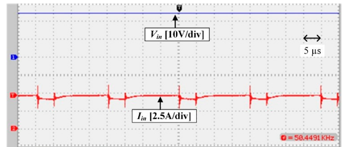
Fig. 7. Input voltage and current waveforms of the modified cascaded Z-source high step-up boost converter.
