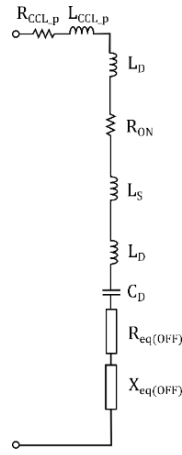
Fig. 5. Equivalent circuit of the load dipole Z_L with discret elements in the HL=10 state.
