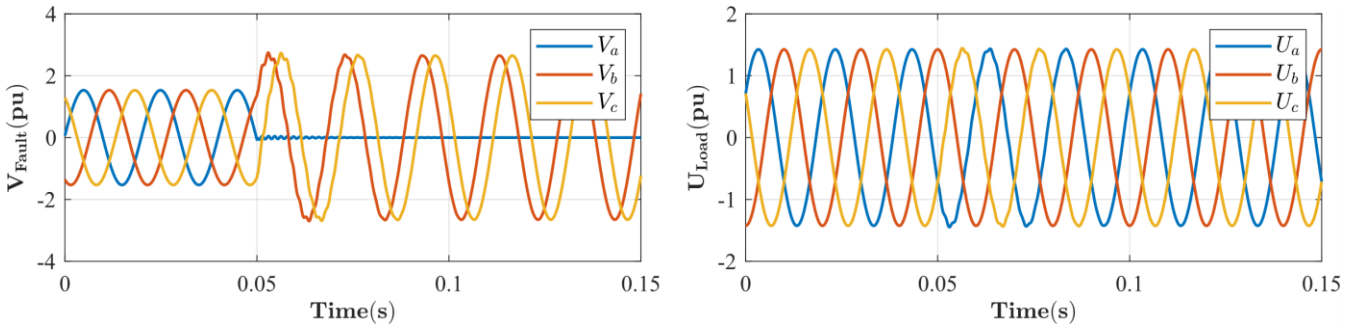
Fig. 5: Phase-to-neutral fault voltages and phase-to-phase load voltages when fault conditions imposed in the fault point at t=0.05 s.
