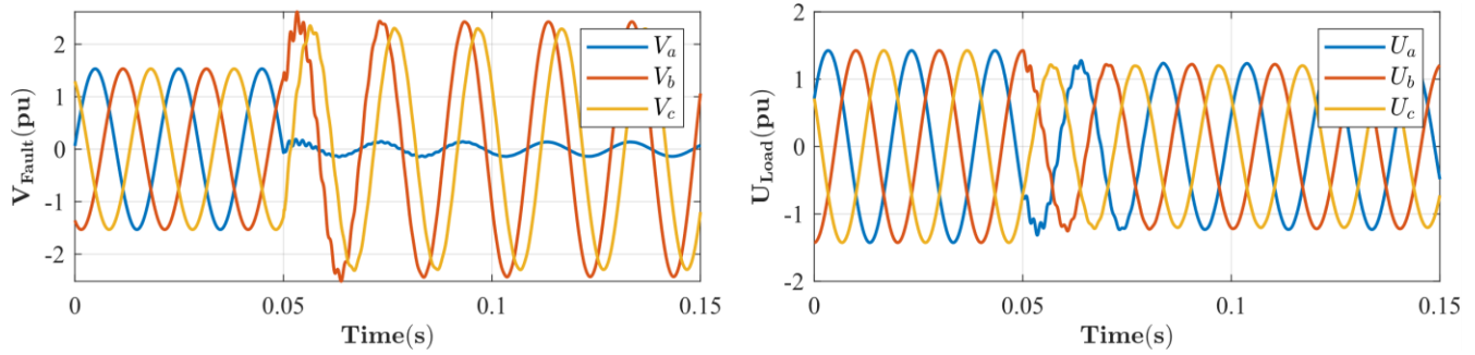
Fig. 4: Phase-to-neutral fault voltages and phase-to-phase load voltages when fault conditions imposed in the MB at t=0.05 s.
