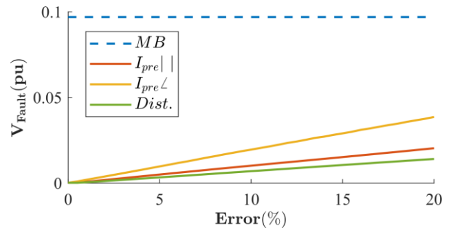
Fig. 7: Measurement errors' effect on fault voltage.
