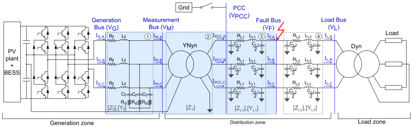
Fig. 2: Considered electrical scheme.
