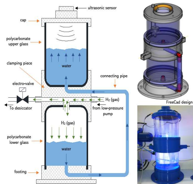
Fig. 6. Gasometer.
