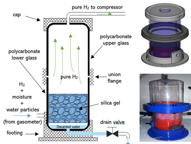
Fig. 7. Desiccator.
