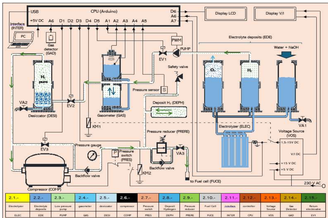
Fig. 10. General scheme of the educational station.
