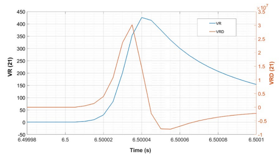
Fig. 11. P2G fault in DC bus 2 R_f=2\ \Omega R 21.
