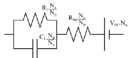
Fig.4. Equivalent circuit of the electrolyzer [16].
