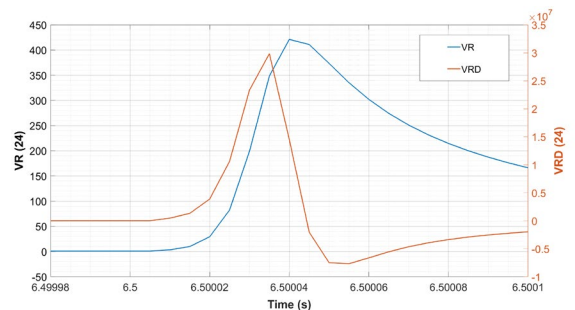
Fig. 12. P2G fault in DC bus 2 R_f=2\ \Omega R 24.
