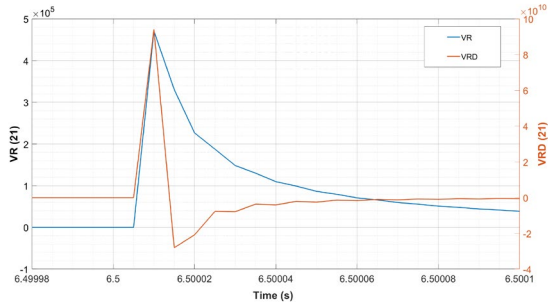
Fig. 7. P2P fault in DC bus 2 R_f=0.01\ \Omega R 21.
