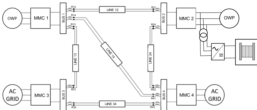
Fig. 3. MVDC grid.
