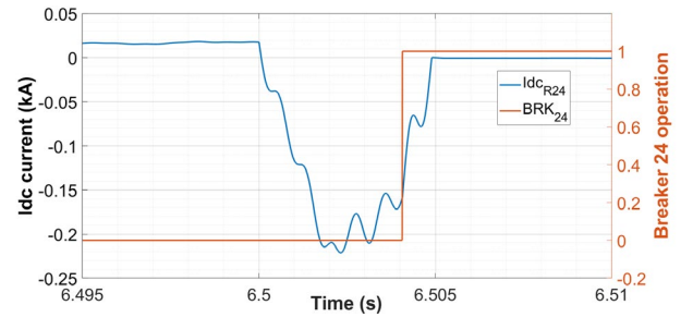
Fig. 10. P2P fault at bus 2 R_f=0.01\ \Omega R 24.
