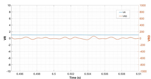
Fig. 6 VR and VRD in steady state.
