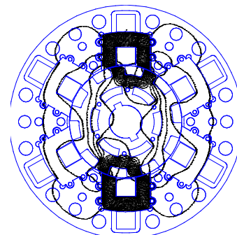
Fig.10. Distribution of magnetic field lines in the SSSRM Al
