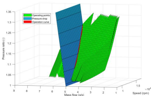
Figure 9. 3D graphic of the operation curve (intersection).
