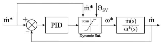
Figure 11. Mass flow control scheme with dynamic saturation.
