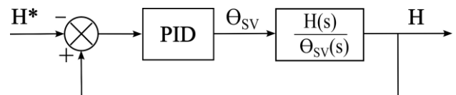
Figure 8. Air humidity regulation scheme.
