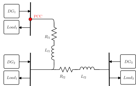
Fig. 5. General schematic of the MG test system.
