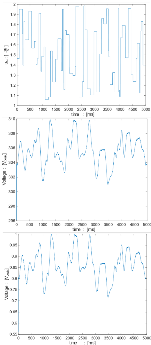
Fig. 4. Response curves from top to bottom: (a) u_v , (b) the generated voltage response, and (c) the pre-processed voltage signal to train the model NN.
