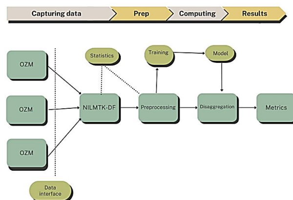
Fig. 2. NILMTK flow diagram.
