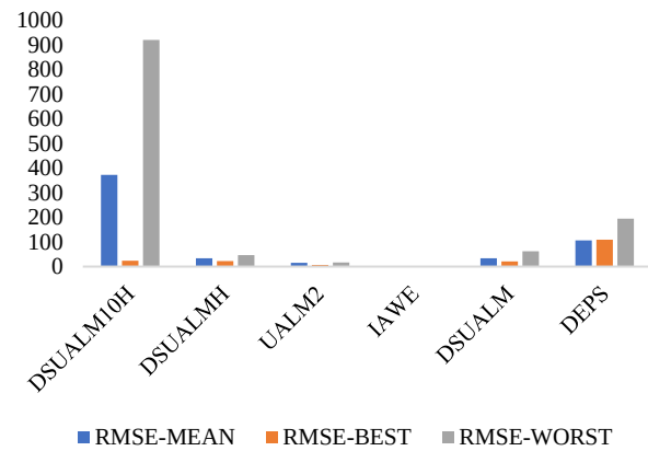
Fig. 9. RMSE metric comparison using the mean, best or worst value.
