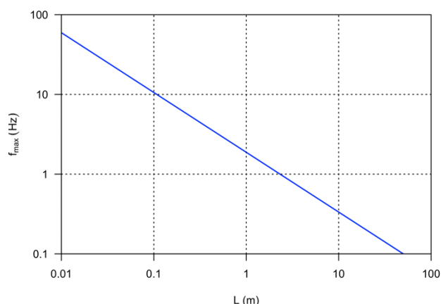
Figure 3. Maximum accessible fluctuation frequency for a given device response length.
