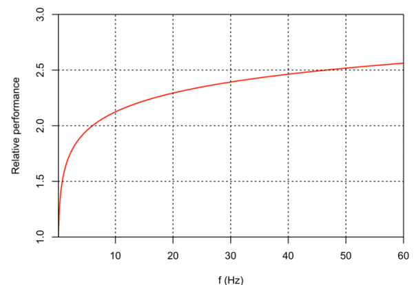
Figure 2. Potential enhancement from additional turbulent energy captured over large HAWT.
