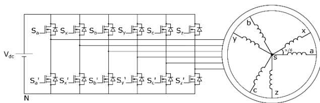
Fig. 1: Block Diagram of the multiphase GaN-based drive.
