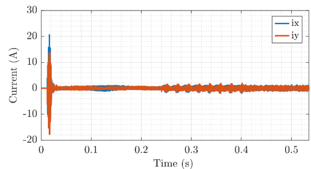
Fig. 11: Currents in xy -plane for the implemented variable switching frequency control.
