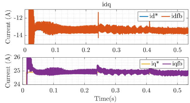
Fig. 10: Current in dq axis ( i_{dq} ) for the three analysed working points.
