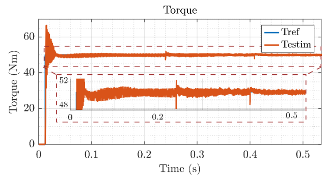
Fig. 6: Simulation results of the torque reference (blue) and torque of the AS6IPMSM (red) for the implemented variable switching frequency control.
