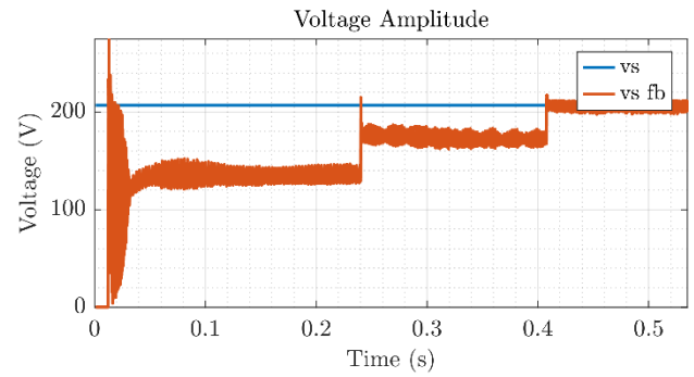
Fig. 9: Maximum voltage amplitude of the machine (blue) and estimated voltage amplitude of the machine (red).
