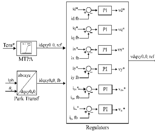
Fig. 2: Block diagram of the control for A6IPMSM and GaN-based drive.
