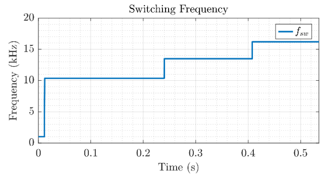
Fig. 5: Selected switching frequency for the implemented variable switching frequency control.
