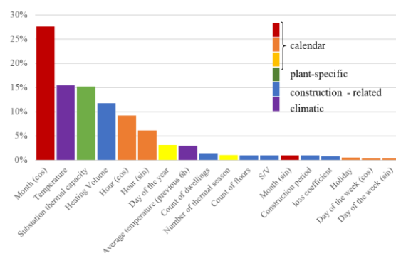
Fig. 5. Model features importance
