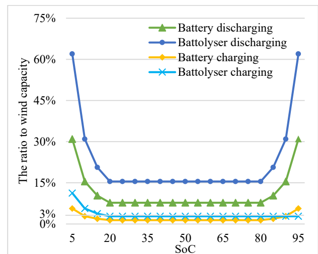
Fig 3. Distribution by SoC of power required by battolyser and battery for PF C in contingencies (wind energy penetration = 30%).
