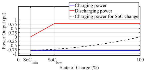
Fig. 1 Output power limits of battolyser
