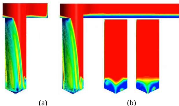
Figure 7. Water volume fraction simulation; (a) all channel, (b) Vertical plane of the basin
