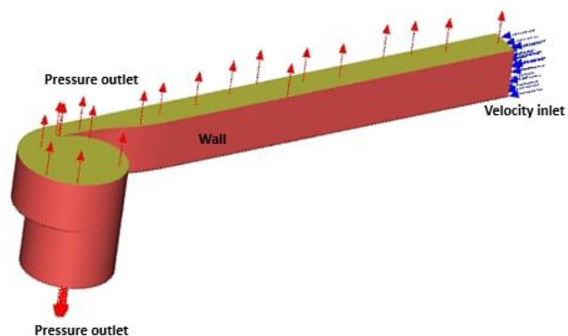
Figure 4. Computational domain and boundary conditions
