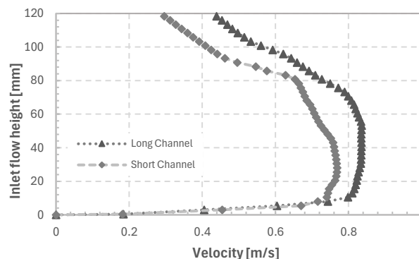
Figure 8. Velocity profile to the basin inlet
