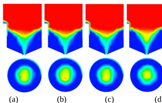
Figure 9. Water volume fraction for H/D=0.5 ; (a) L_c/D = 0.9 y w_2/D=0.4 , (b) L_c/D = 0.7 y w_2/D=0.6 , (c) L_c/D = 0.9 y w_2/D=0.6 y (d) L_c/D = 0.7 y w_2/D=0.4
